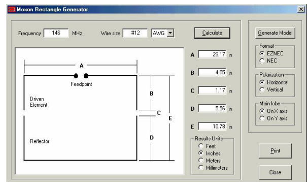
Figure 1. Screenshot of the Moxon Rectangle Generator (courtesy AC6LA)
