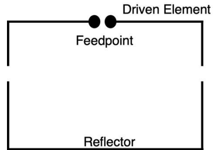
Fig 1-Basic layout of the Moxon rectangle antenna
